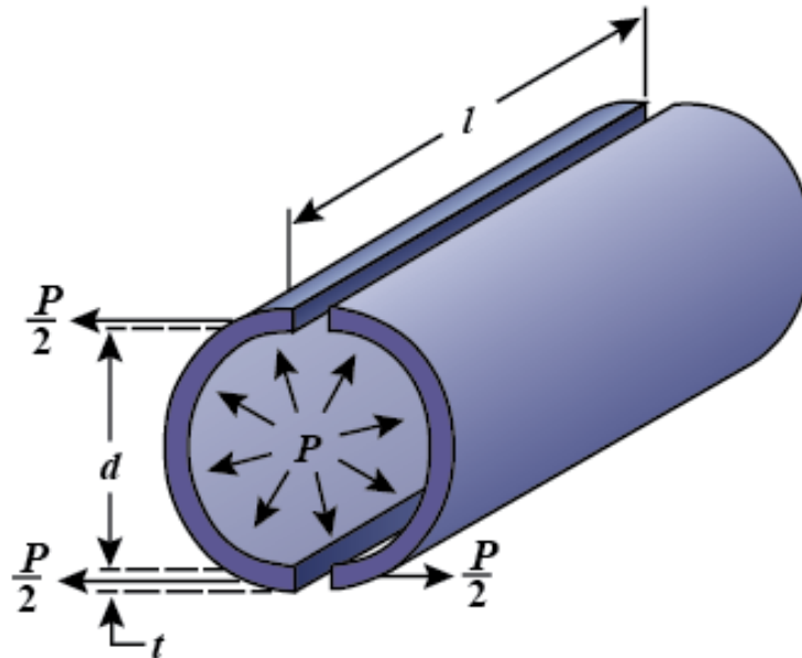
Figure 6.2b: Circumferential forces acting on thin cylinder (internal pressure)
