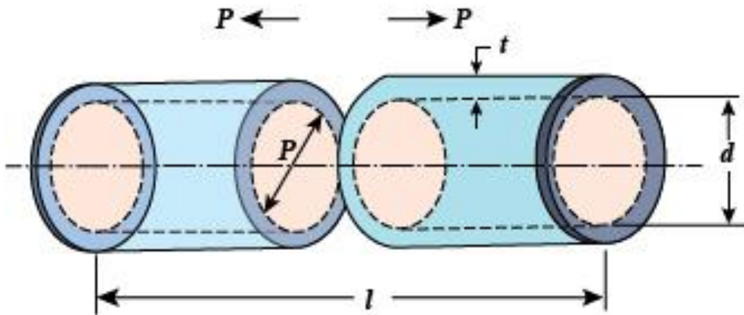
Figure 6.2a: Longitudinal forces acting on thin cylinder (internal pressure)
