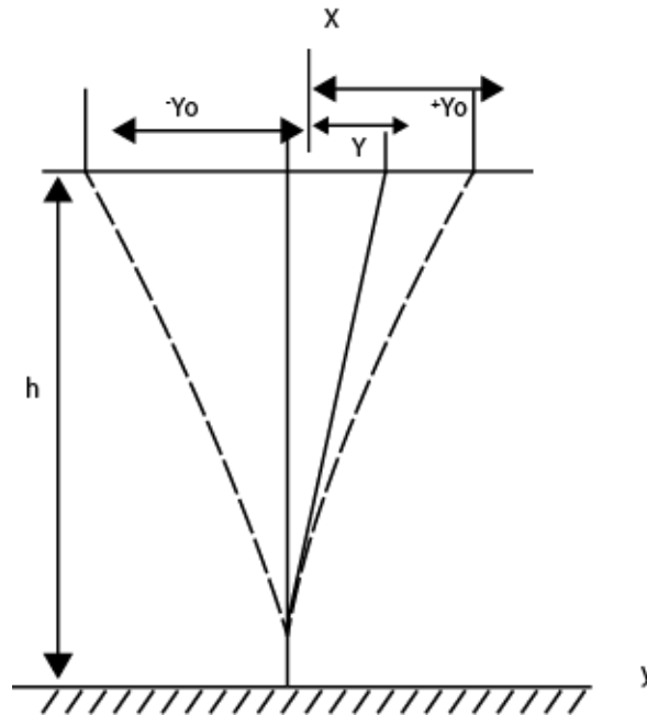
Figure 6.4b: Seismic forces on tall column
