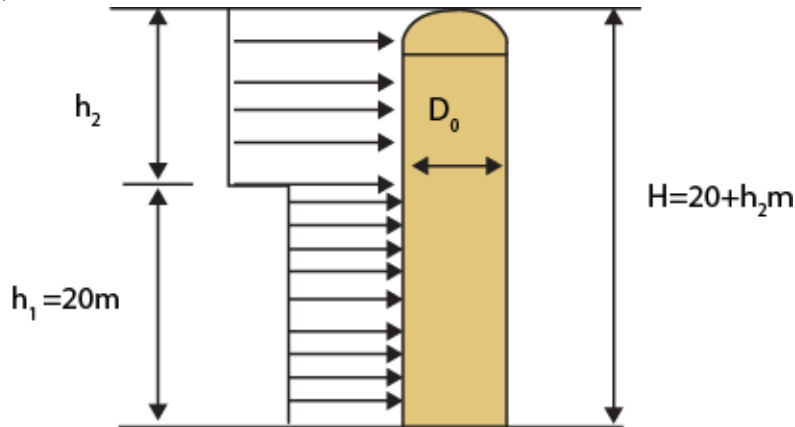
Figure 6.3: Tall column subjected to wind pressure
