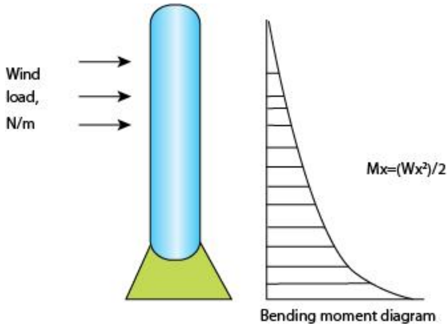
Figure 6.1: Bending moment diagram under wind load
